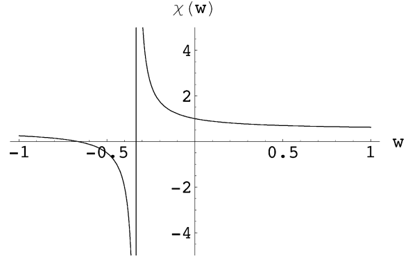
Figure 1. The \chi -factor (53) as a function of w in the commonly discussed range w \in [-1, 1] . Naturally \chi(0) = 1 , which corresponds to the Newtonian case, see equations (48)–(50). At the ends of the plotted range we find \chi(-1) = 1/4 and \chi(1) = 5/8 . The zero-crossing and the first-order pole correspond to w = -2/3 and -1/3 , respectively, as is obvious from equation (53).
