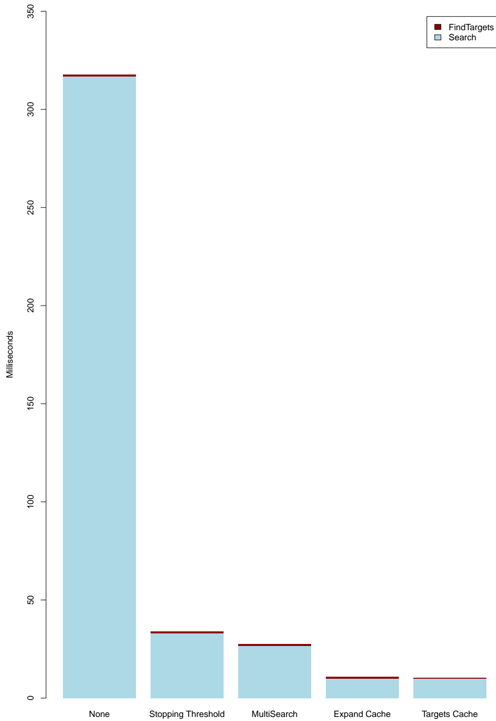
Figure 5.3: Average processing time per input for WordSub optimisations.
